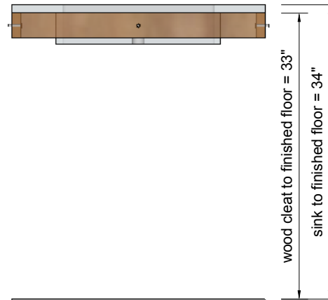
Back view showing placement of wood cleats
