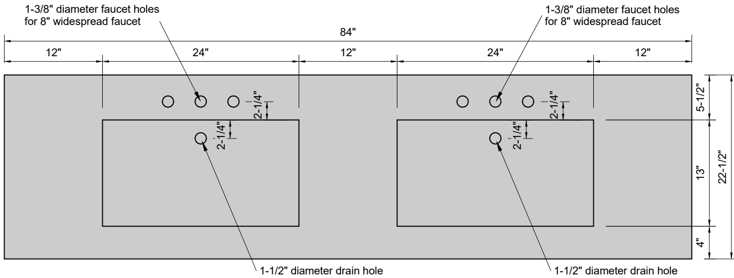
TOP VIEW
