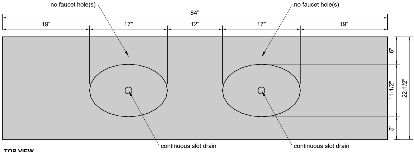
TOP VIEW
