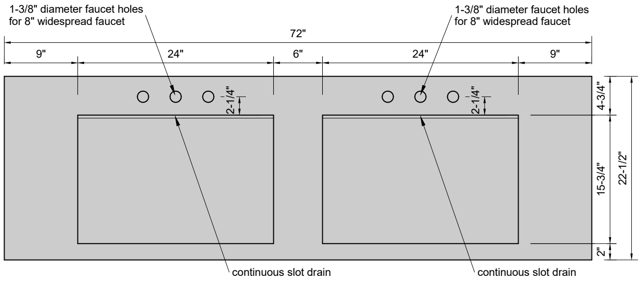
TOP VIEW
