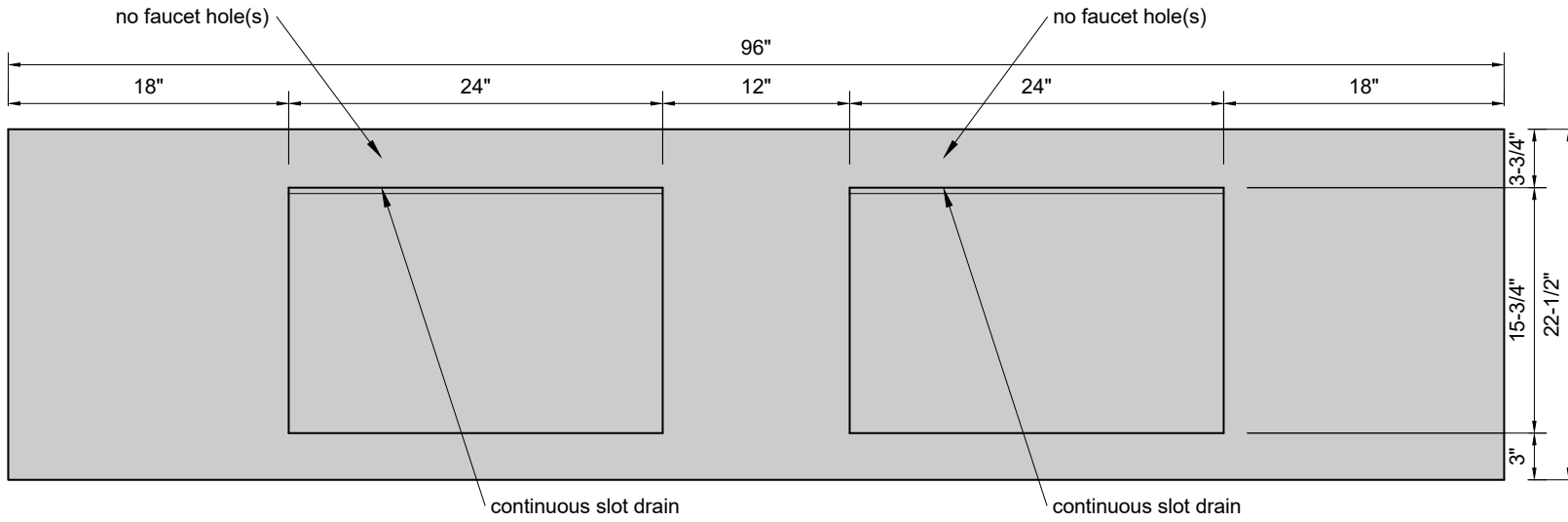
TOP VIEW
