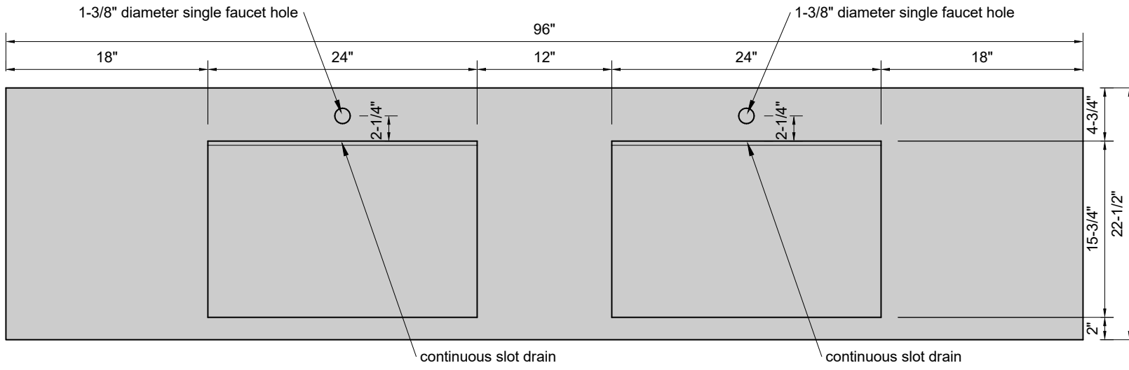
TOP VIEW
