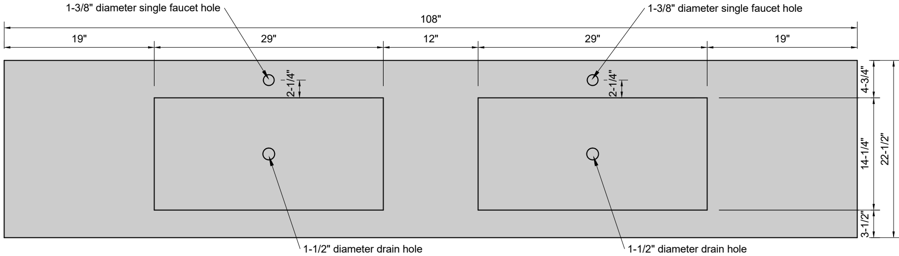
TOP VIEW
