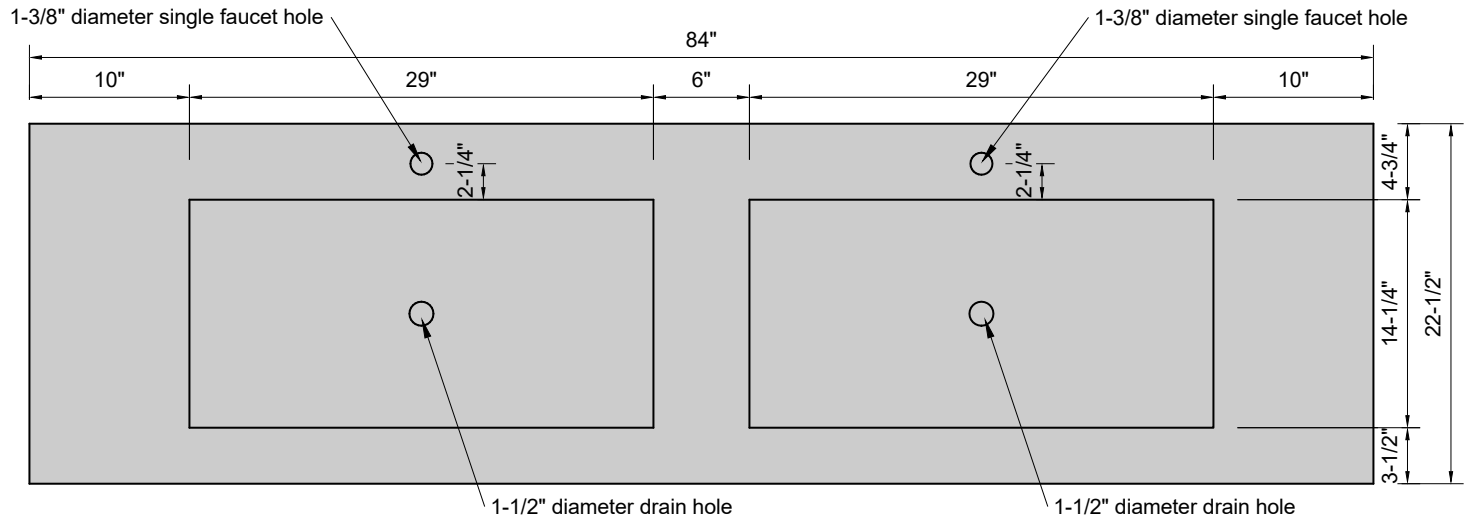
TOP VIEW
