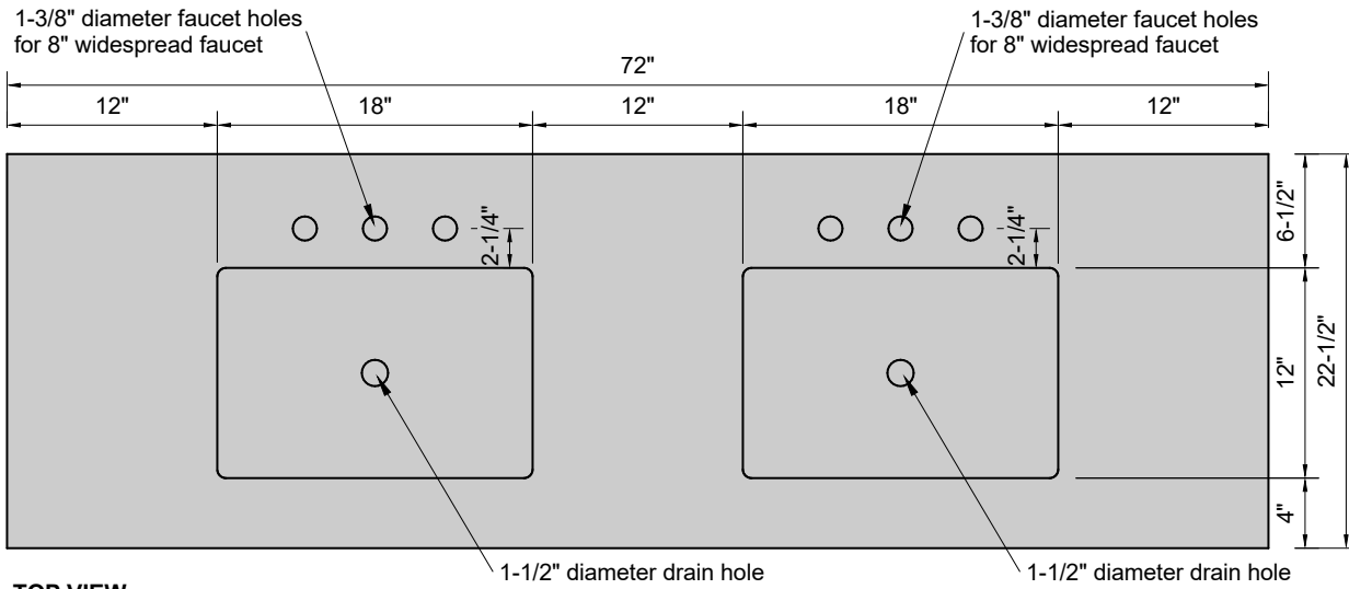
TOP VIEW
