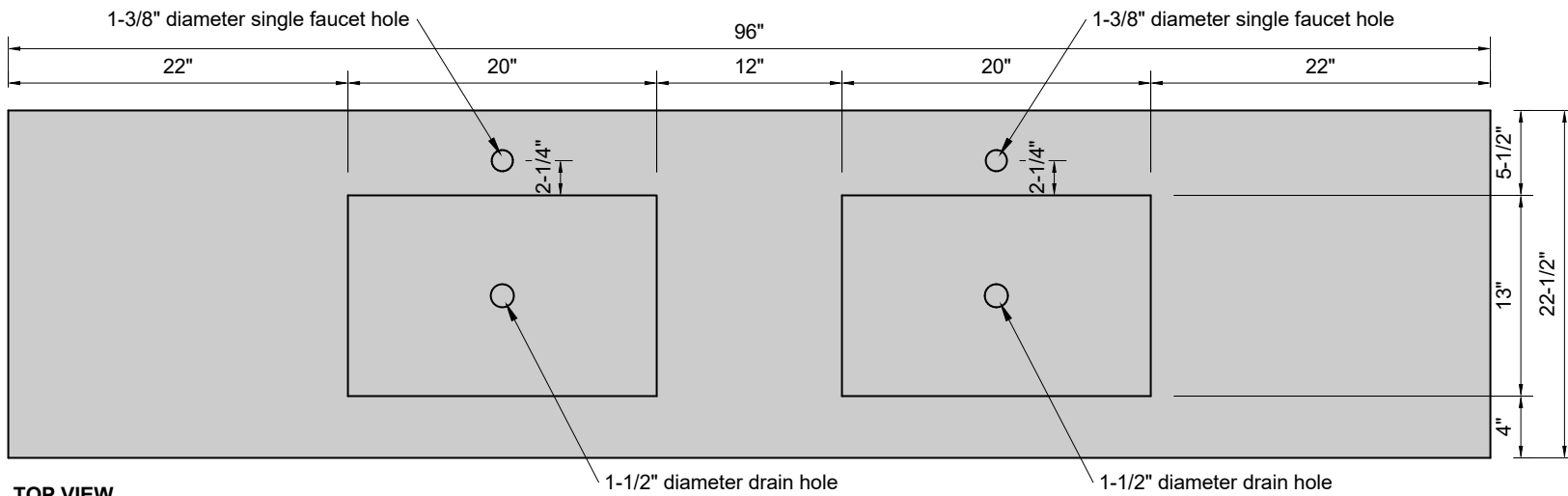
TOP VIEW
