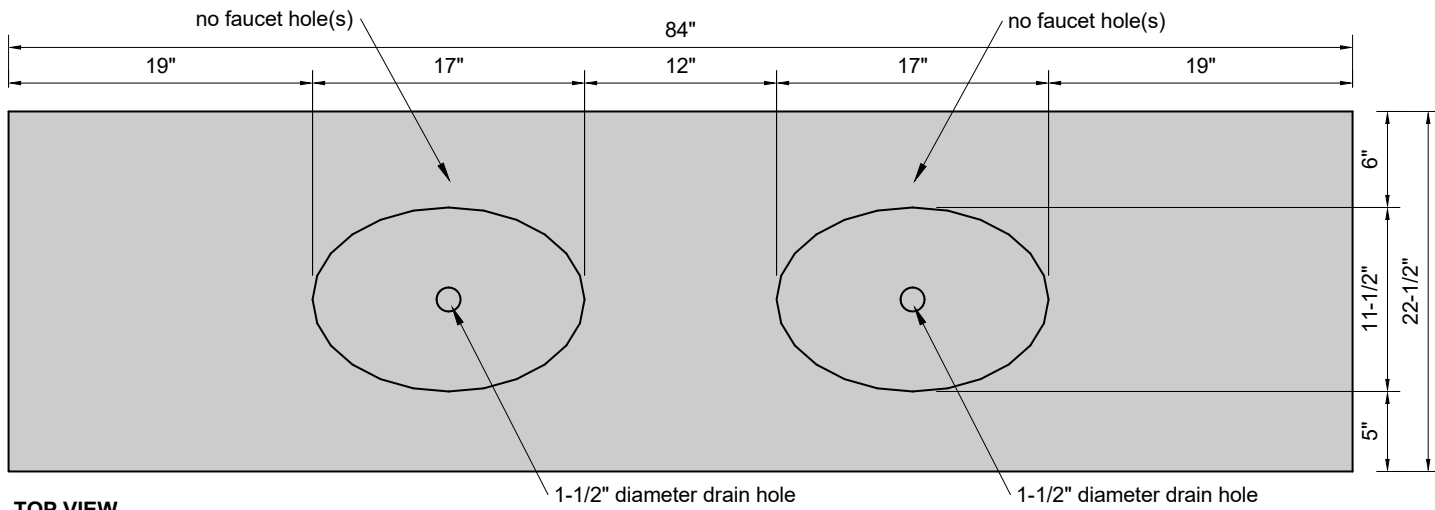
TOP VIEW
