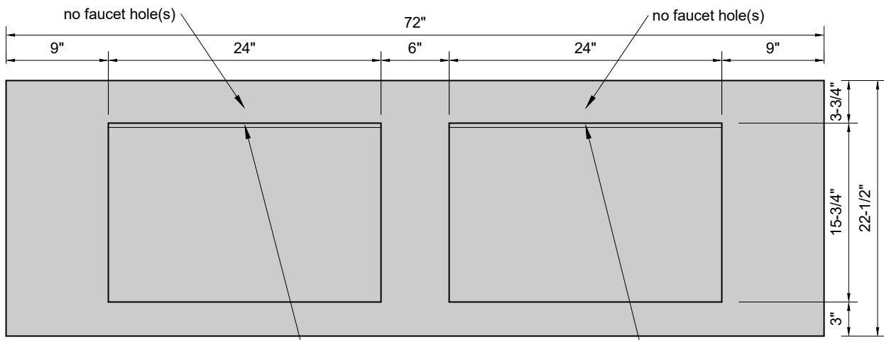
TOP VIEW
