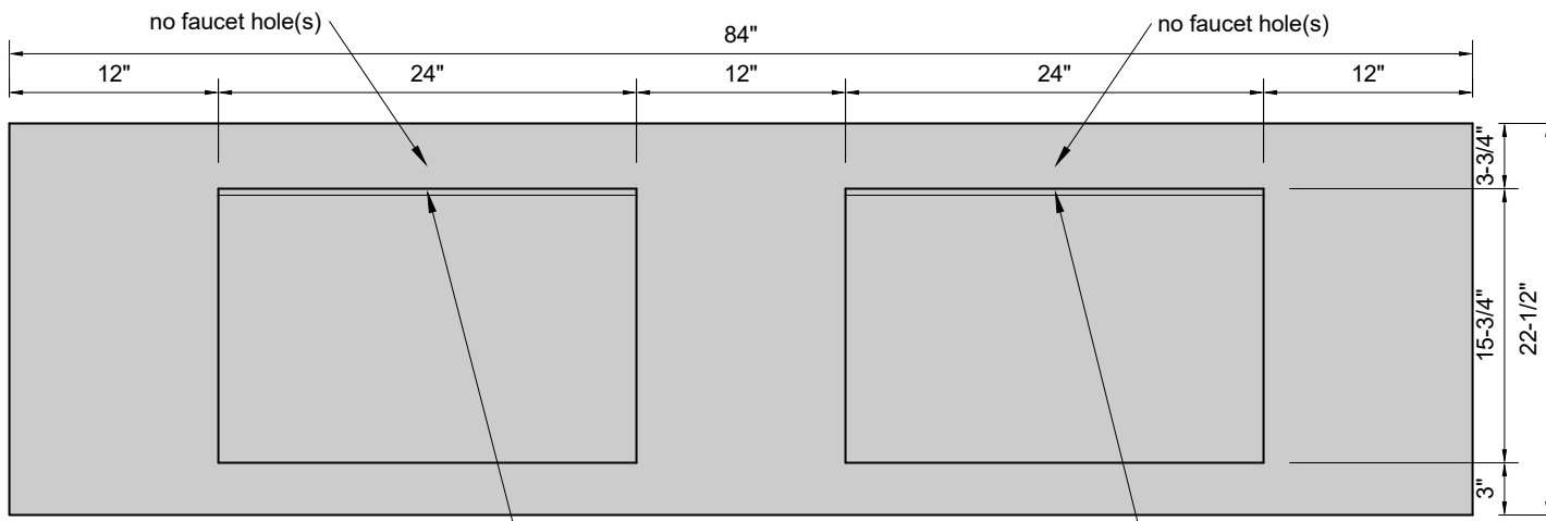
TOP VIEW
