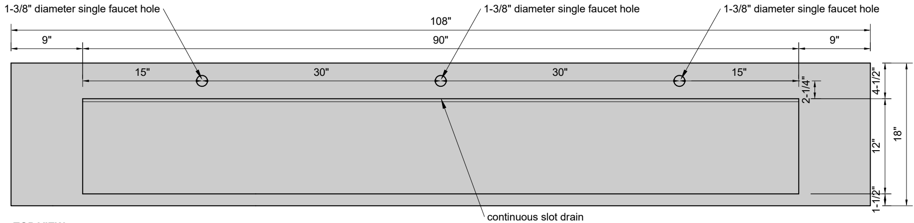
TOP VIEW
