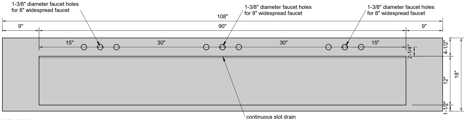
TOP VIEW
