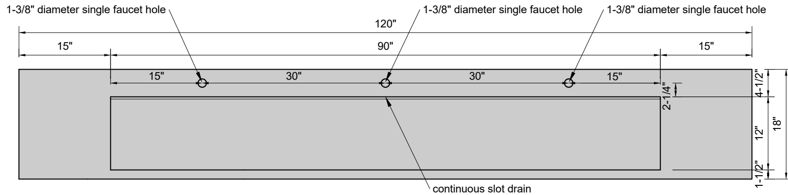
TOP VIEW
