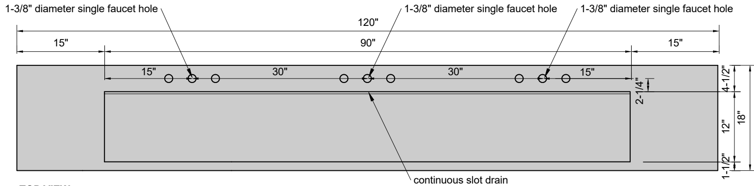
TOP VIEW
