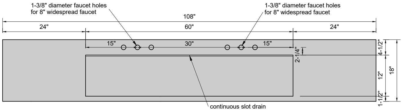
TOP VIEW
