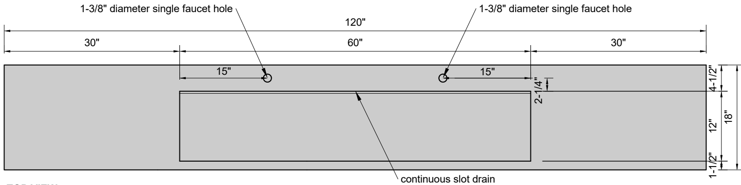
TOP VIEW
