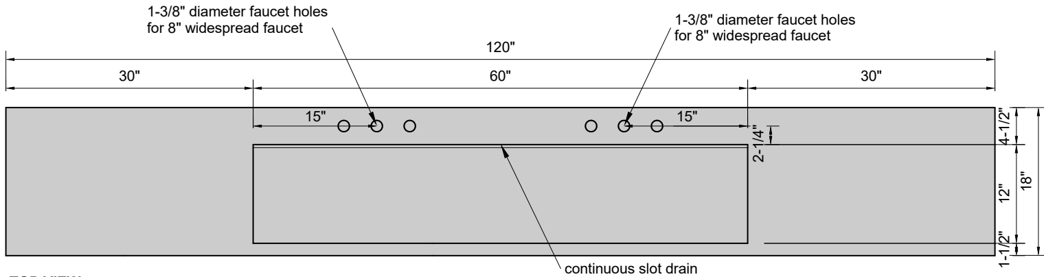
TOP VIEW
