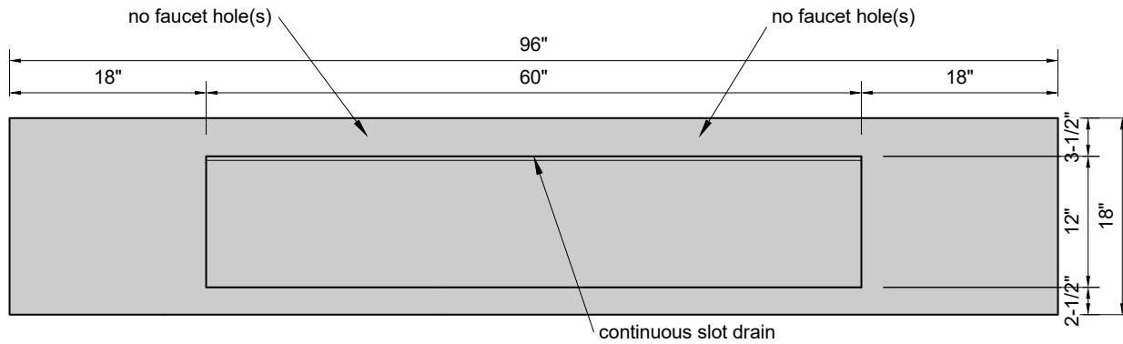
TOP VIEW
