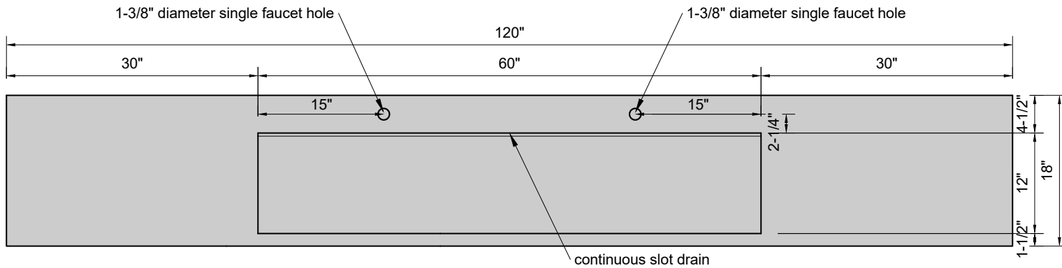
TOP VIEW
