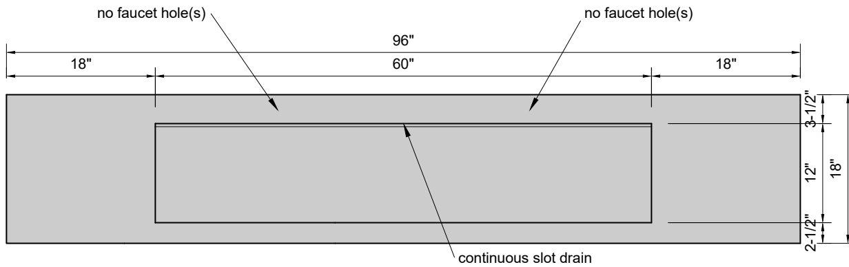
TOP VIEW
