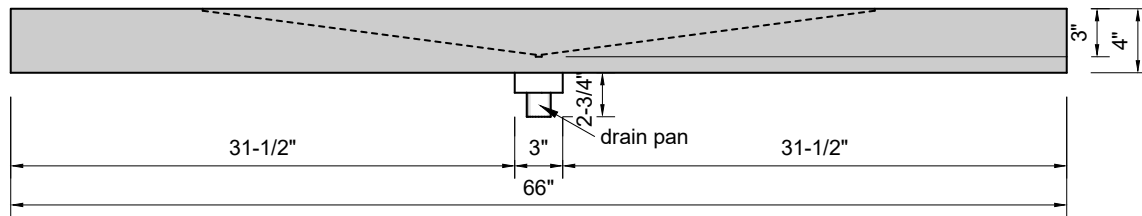
FRONT VIEW
