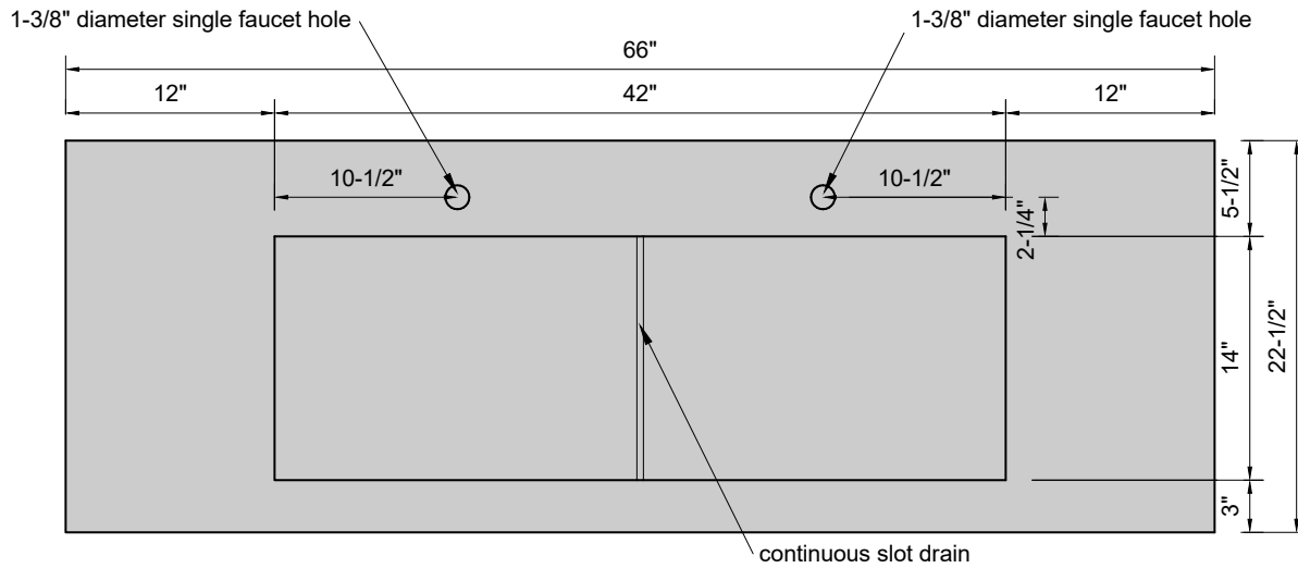
TOP VIEW
