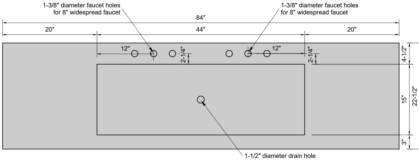
TOP VIEW
