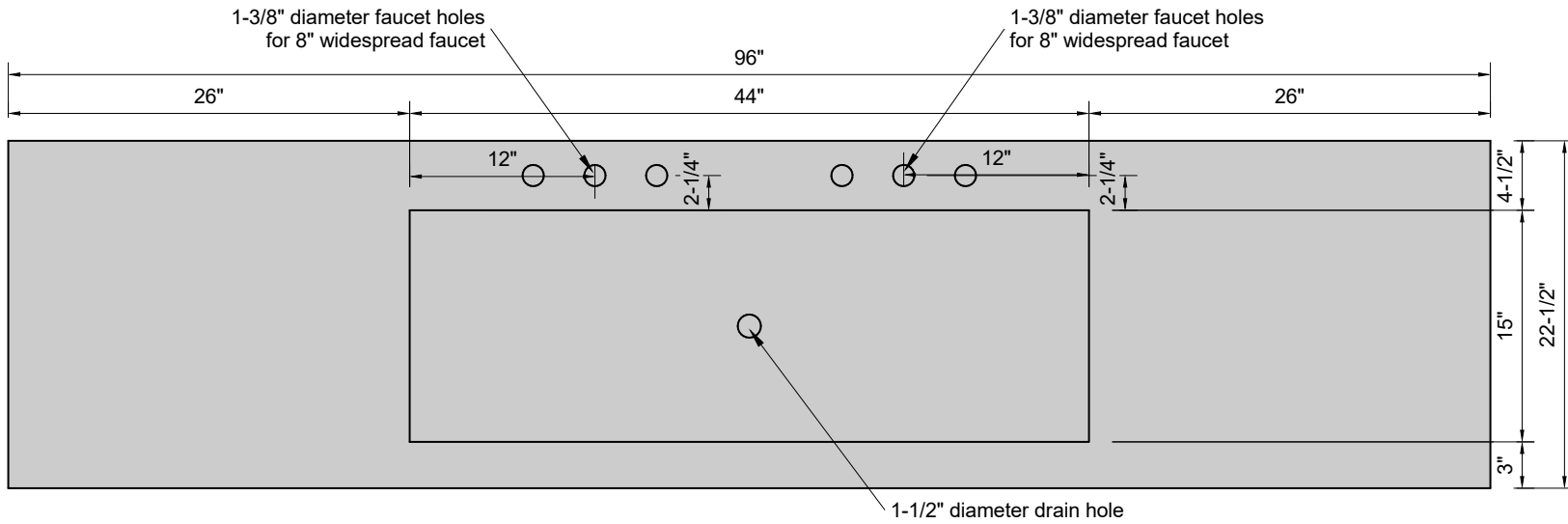
TOP VIEW
