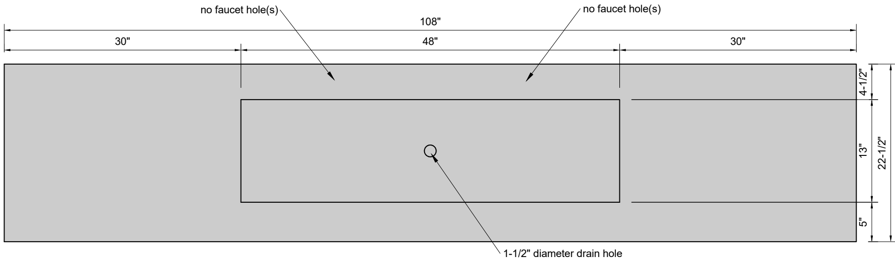
TOP VIEW
