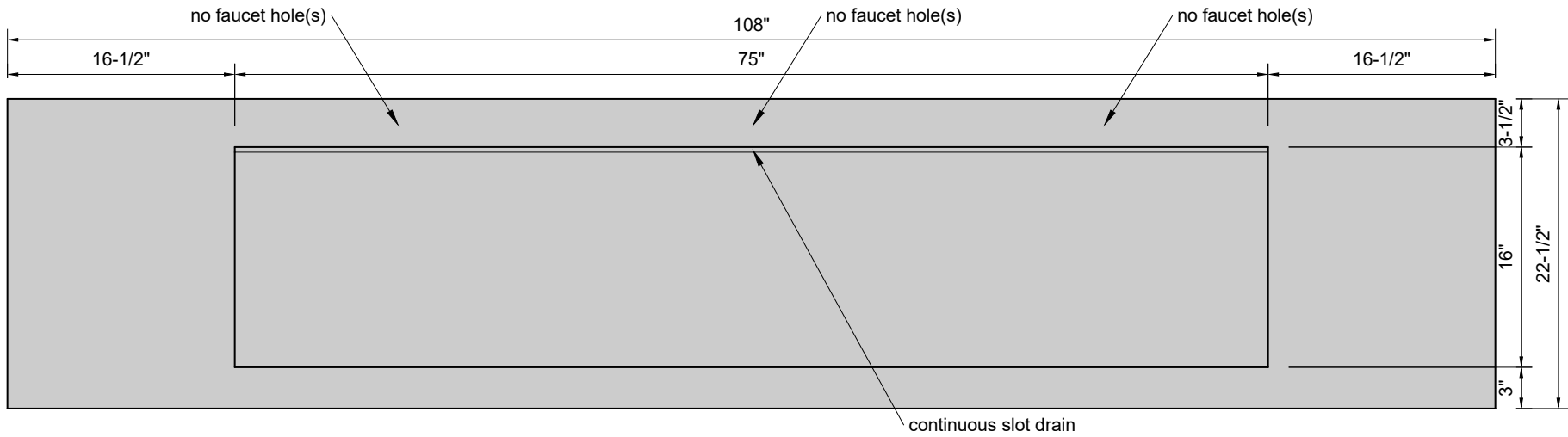
TOP VIEW
