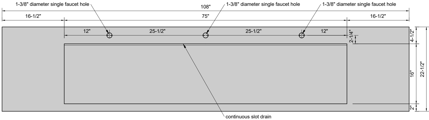
TOP VIEW
