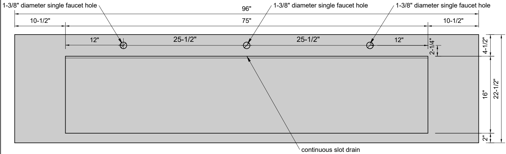
TOP VIEW
