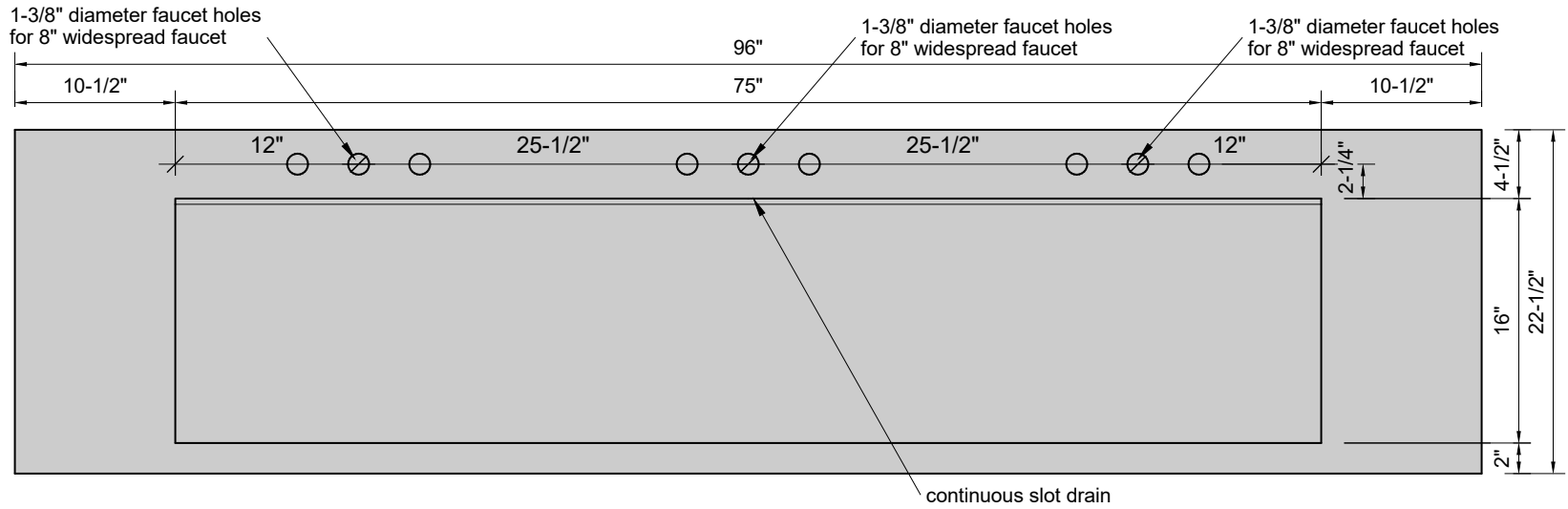
TOP VIEW
