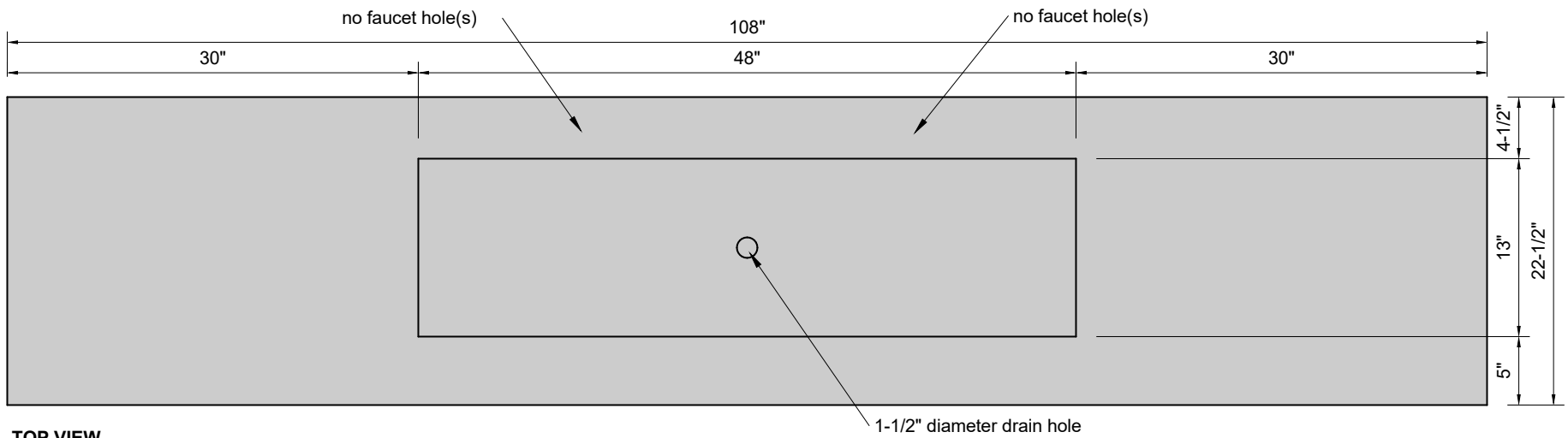
TOP VIEW
