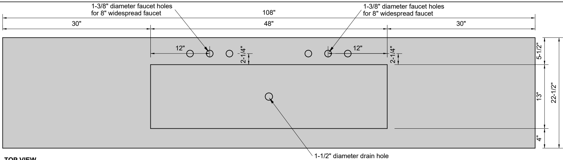
TOP VIEW
