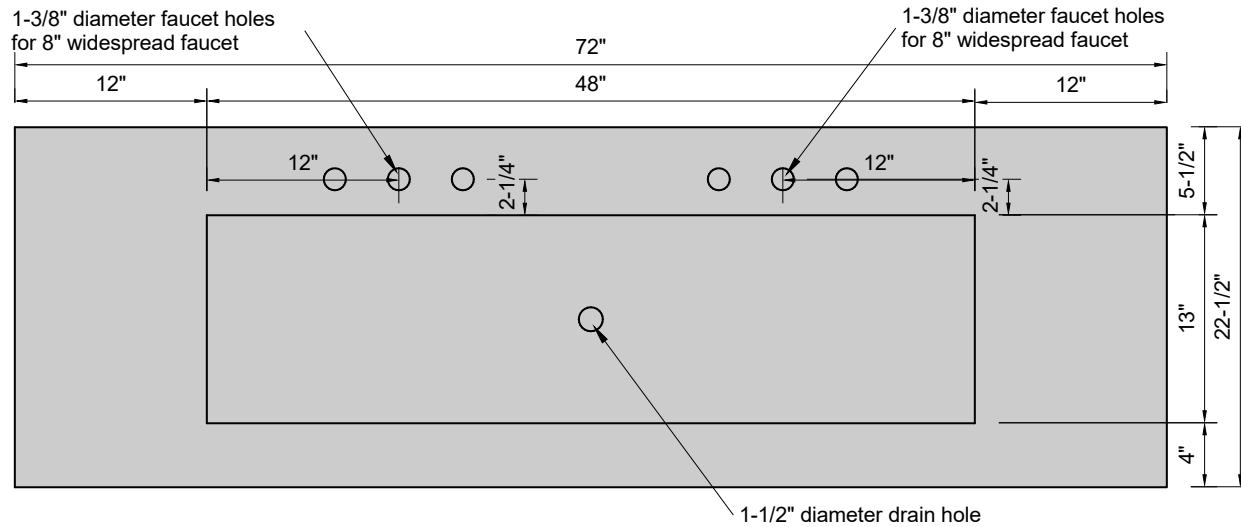
TOP VIEW
