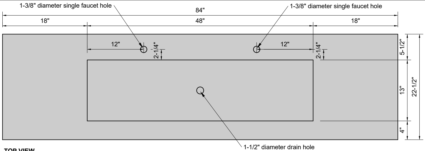
TOP VIEW
