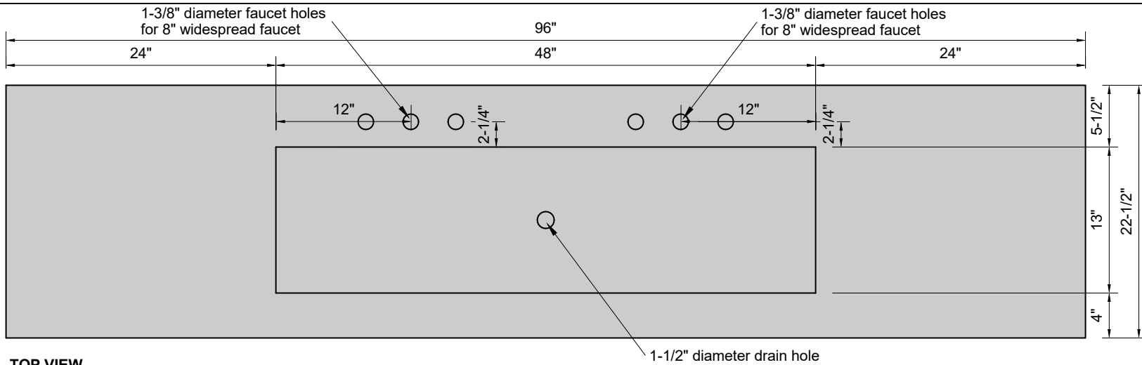
TOP VIEW
