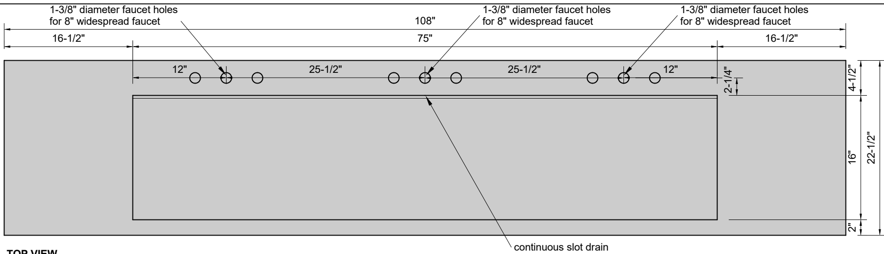
TOP VIEW
