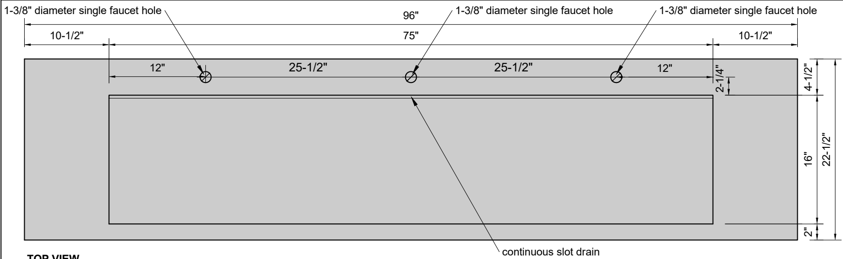
TOP VIEW
