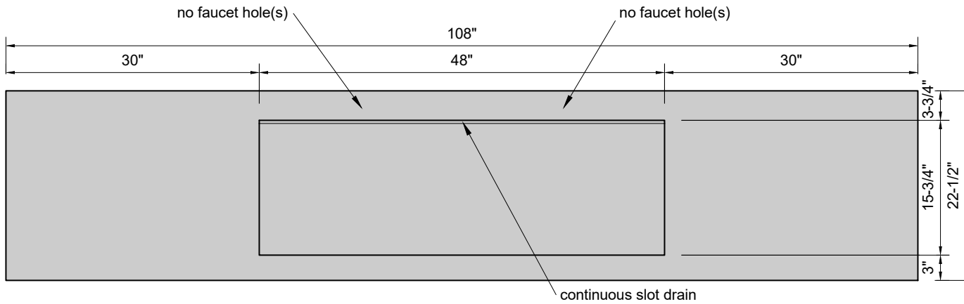
TOP VIEW
