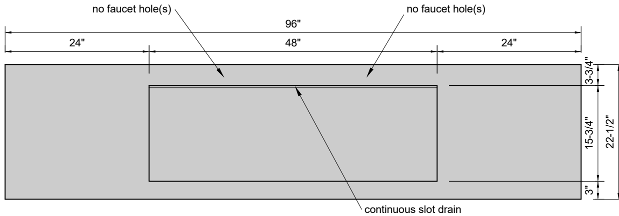
TOP VIEW
