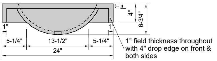
BACK VIEW
