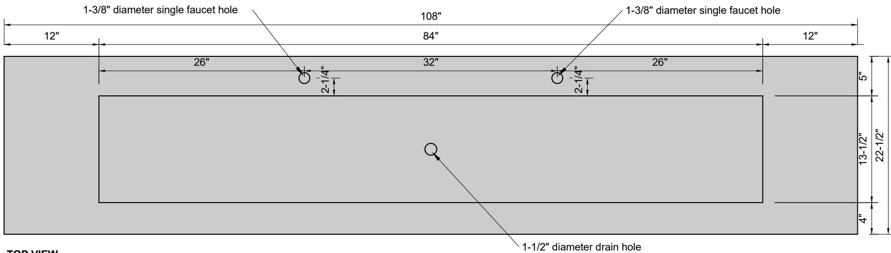
TOP VIEW
