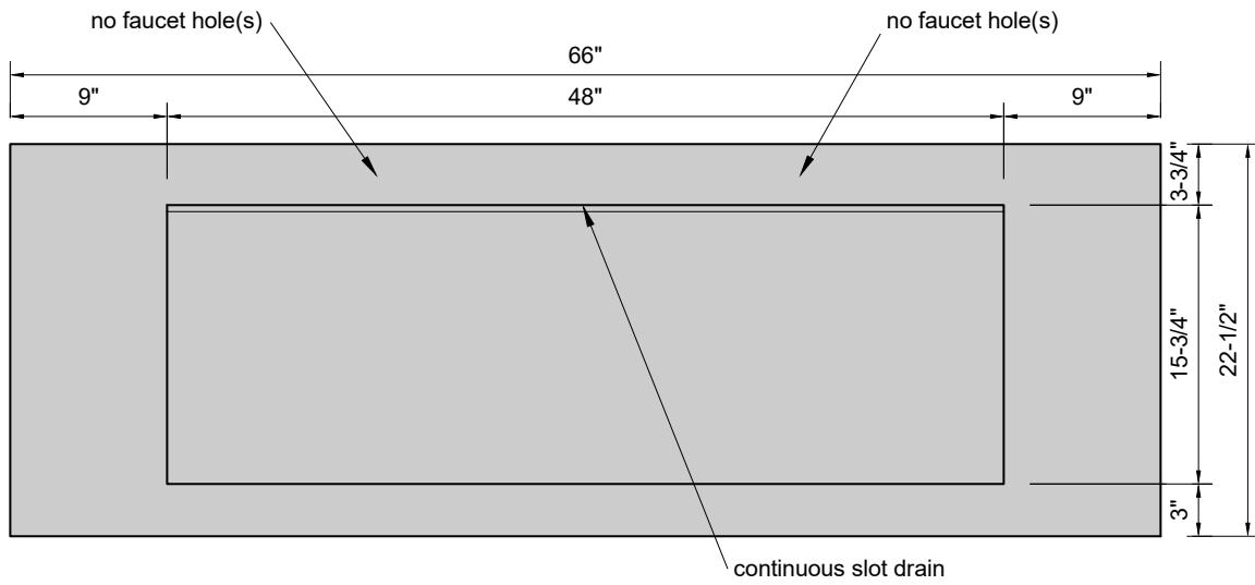
TOP VIEW
