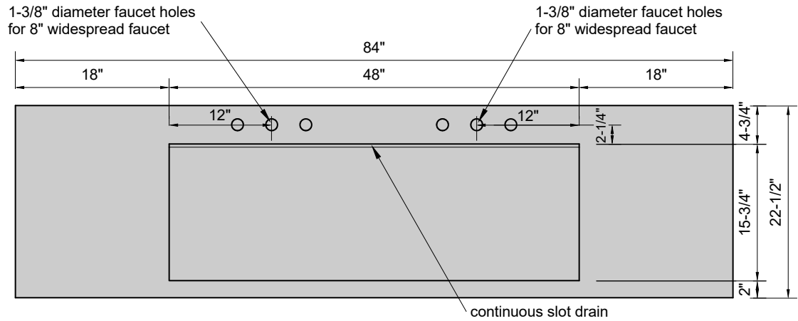
TOP VIEW
