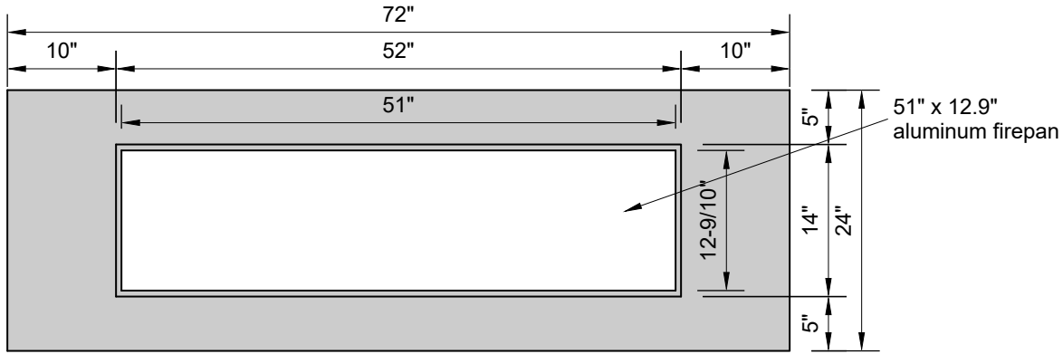
TOP VIEW
